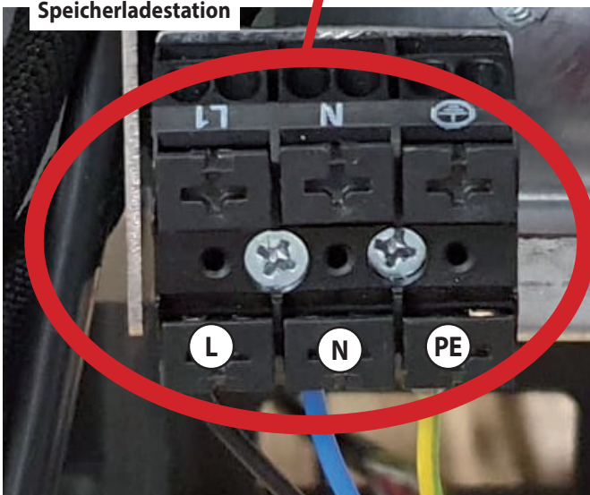
Anschlüsse Pumpe Speicherladestation
